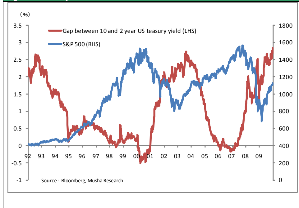
Figure 2 : The yield curve and S&P 500
